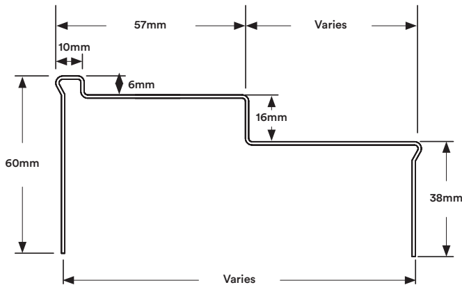
ISD Frame to suit 57mm Door
