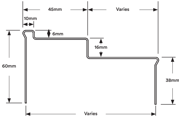
ISD Frame to suit 45mm Door
