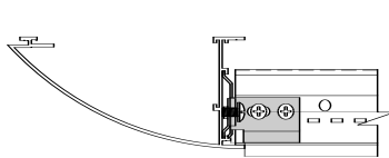
Profiled AXIOM with Tegular Edge panel
