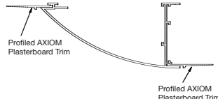
Profiled AXIOM with Plasterboard Trim (AXDWT)
