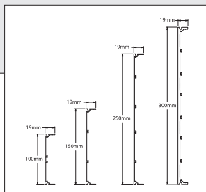
Classic AXIOM Trim profiles
