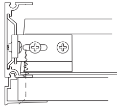
Classic AXIOM with Plasterboard Trim (AXBT)
