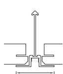
Beveled Tegular with K2C2 Edge and Top Hat Grid
